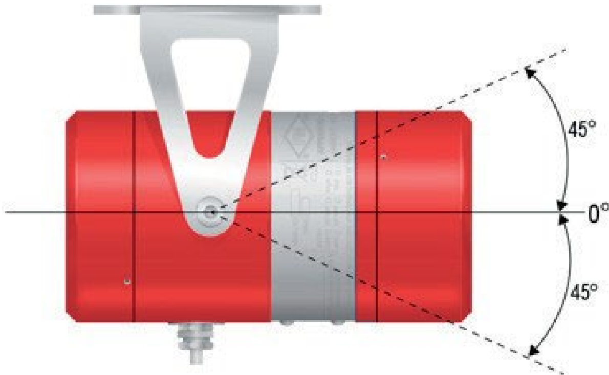
Figure 3: Wall Mount
