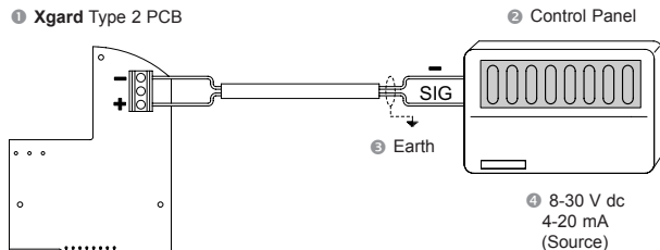
Diagram 10: Xgard Type 2 electrical connections
